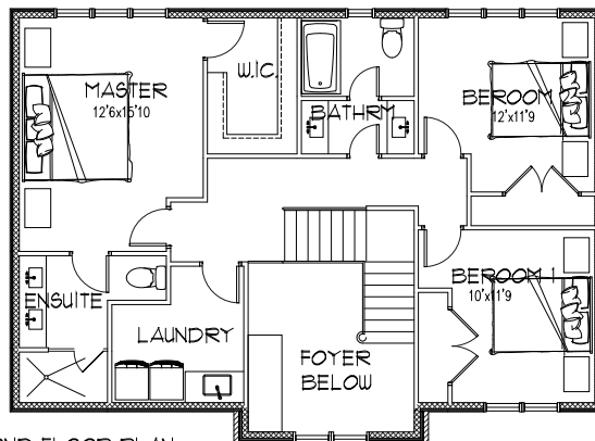
SECOND FLOOR PLAN 993 SQFT
