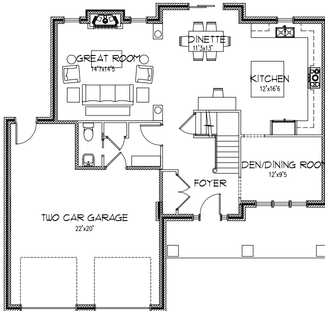
MAIN FLOOR PLAN 1092 SQFT
