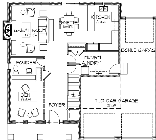
MAIN FLOOR PLAN 1061 SQFT
