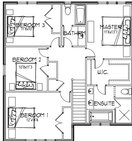
SECOND FLOOR PLAN 1131 SQFT
