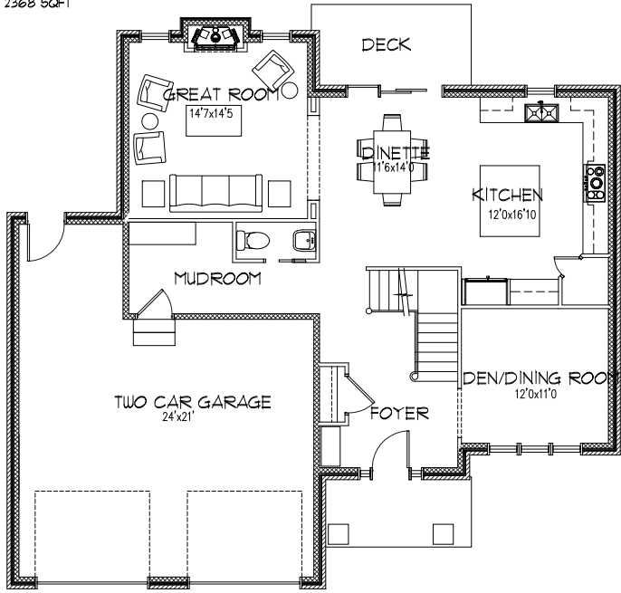
MAIN FLOOR PLAN 1166 SQFT
